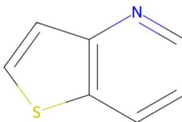
Figure 1: 2D structure of Thienopyridine
