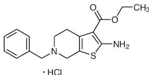
Figure 2: 2D structure of Tinoridine Hydrochloride
